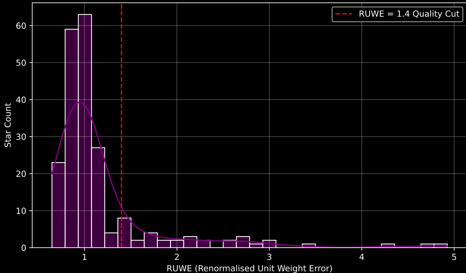
GALAH DR4 Field [7123] RUWE Distribution (n= 211)
