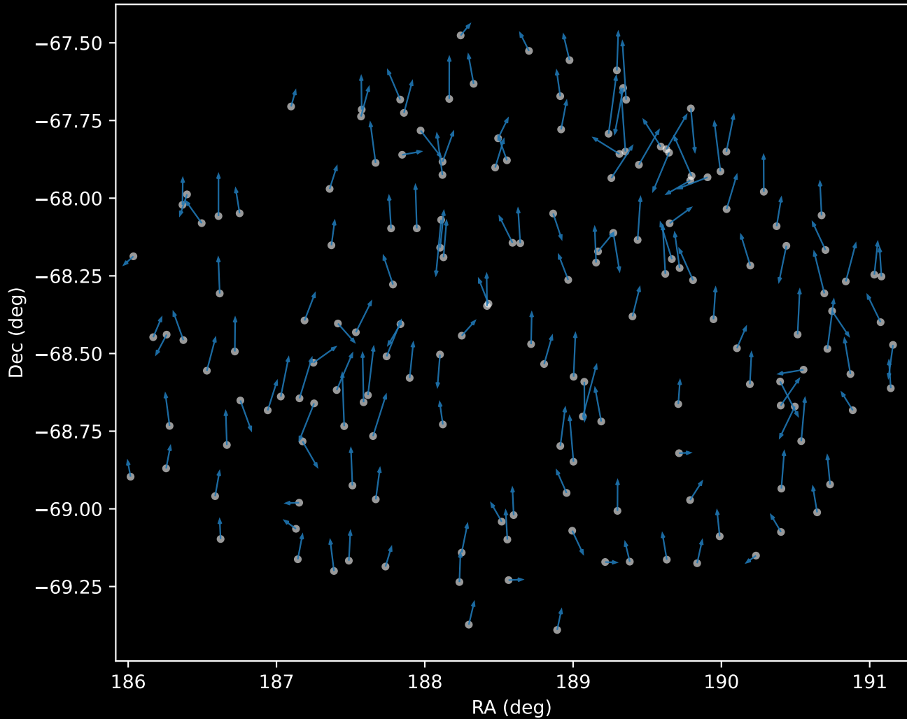
GALAH DR4 Cluster 0 Proper Motion Vectors (n=167)
